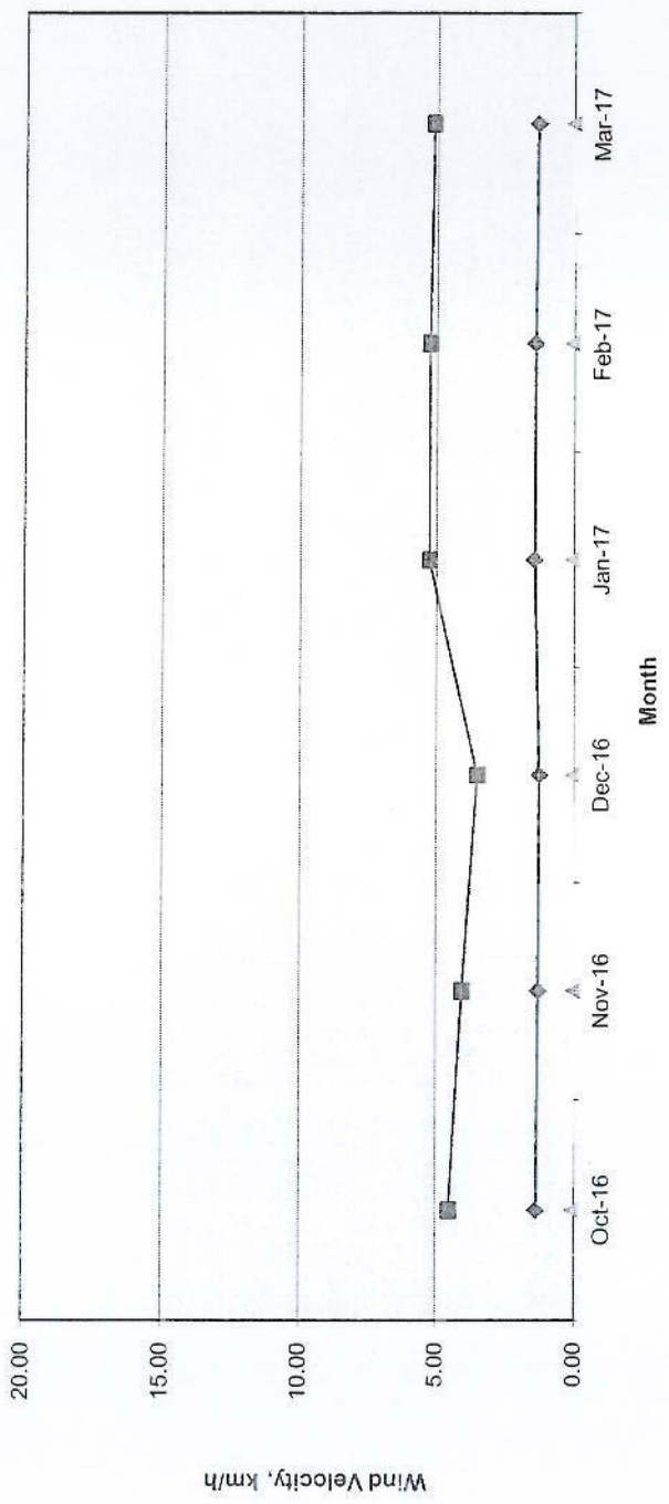
Wind Velocity - Trend Chart Oct-16 to Mar-17
