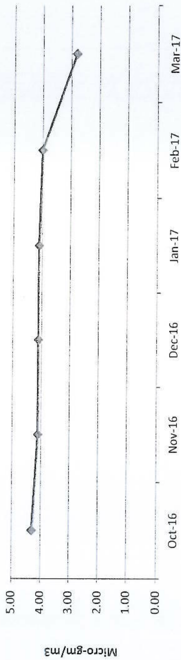
NOx Trend Chart (Oct-16 to Mar-17)
