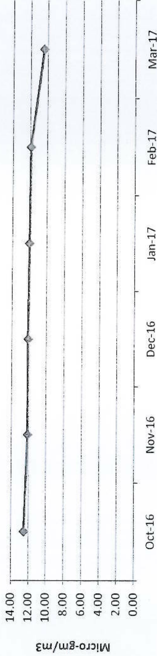
PM2.5 Trend chart(Oct-16 to Mar-17)
