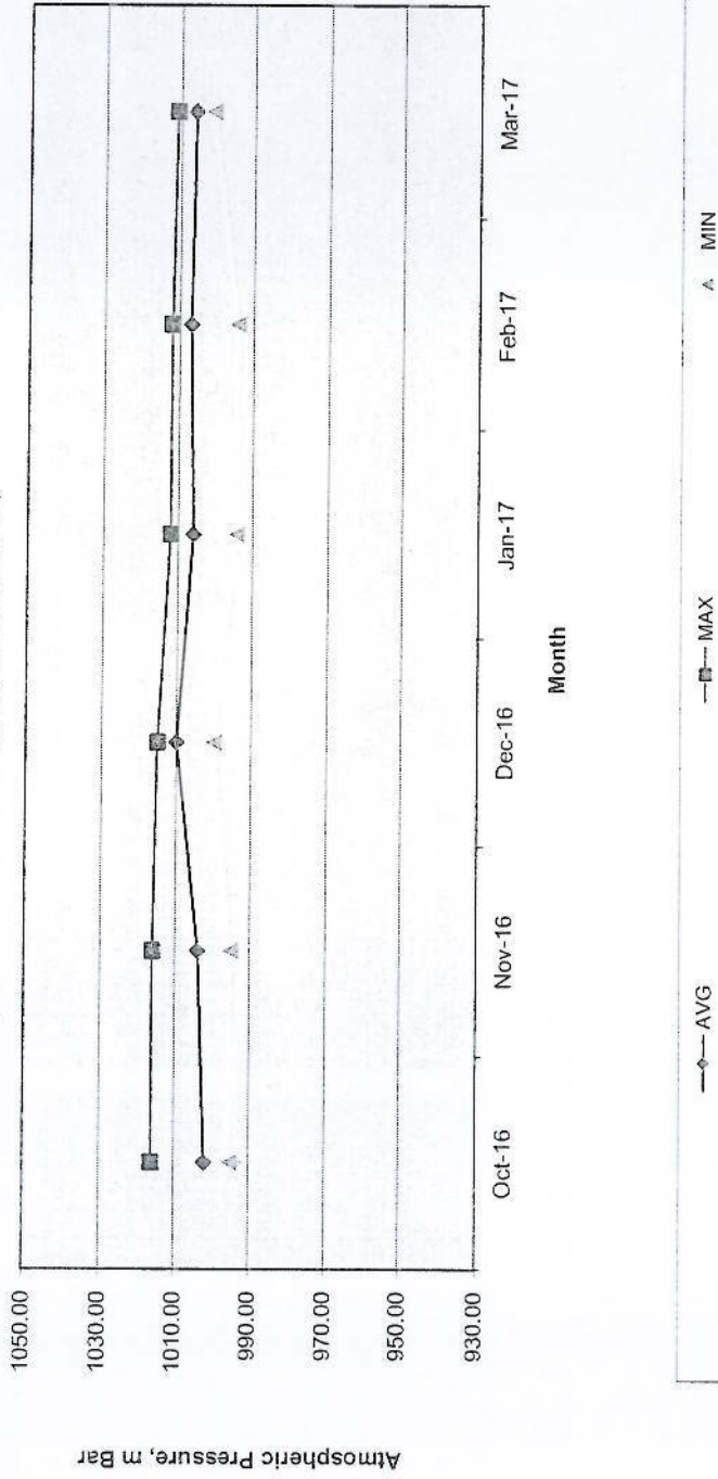
Atmospheric Pressure - Trend Chart (Oct-16 to Mar-17)
